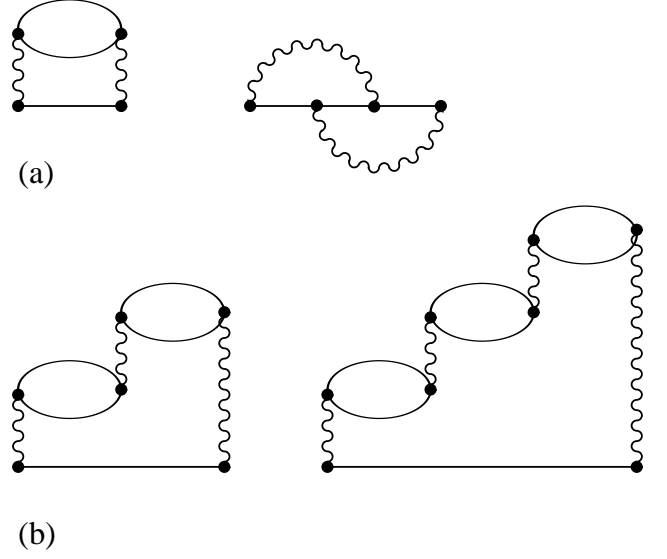
Fig. 4. (a) Green's function diagrams leading to equation (36), similar to Figure 3c. (b) Green's function bubble diagrams leading to equation (97), similar to Figure 3d.
