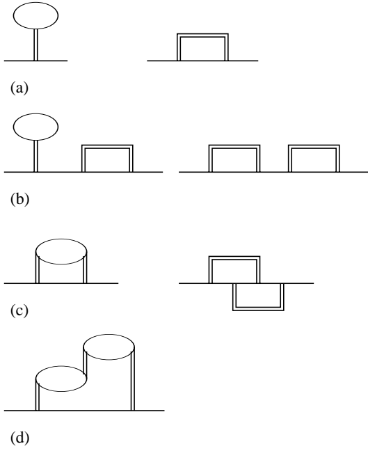
Fig. 3. (a) First order Ursell diagrams; the double line corresponds to one operator U_2 . Here we slightly change the representation of reference [21] and replace the dotted segments there (corresponding to a summation over all exchange cycle lengths) by closed curves; in this way, the U_2 diagrams become very similar to the usual Green's function diagrams. Despite this close graphical similarity, the physical interpretation of the diagrams is different: for instance, exchange cycles do not appear at all in Green's function diagrams. (b) Simplest examples of the diagrams included in the iteration. (c) Diagrams leading to equations (24) and (106). (d) Bubble diagrams leading to equation (109).
