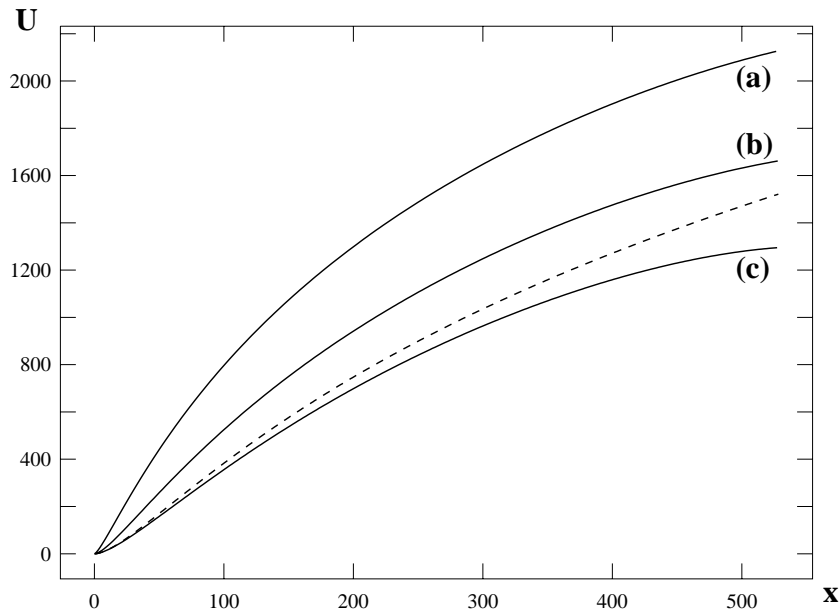
Fig. 5. Self-energy U(k) in units of a^2/\lambda^4 plotted as a function of x = k^2/a for the three approximations discussed in the text: (a) self-consistent one bubble approximation, (b) self-consistent ladder summation, and (c) self-consistent bubble sum. These results are obtained with an ultraviolet cutoff of \Lambda\lambda^2/a \simeq 800 . The dashed line shows the analytical (not self-consistent) calculation of U(k) in the bubble approximation, equation (82).
