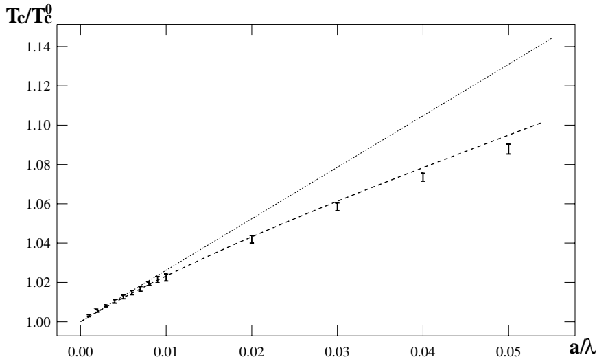
Fig. 6. Dependence of the transition temperature, T_c/T_c^0 , of a dilute homogeneous Bose gas on scattering length a/\lambda , calculated by solving equations (100, 101) self-consistently. The dashed line is a fit to the data points, given by equation (102). The asymptotic linear behavior extracted from this fit is shown for comparison. The linear behavior is seen only at very small values of a/\lambda .
